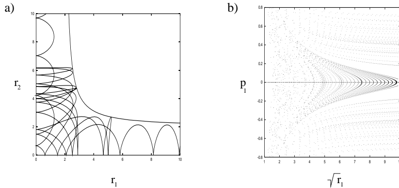
Fig. 6.3 (a) A typical trajectory in the [r_1, r_2] plane; the trajectory enters here along the r_1 axis and escapes to infinity along the r_2 axis; (b) Poincaré map ( r_2=0 ) for collinear helium. Strong chaos prevails for small r_1 near the nucleus.
