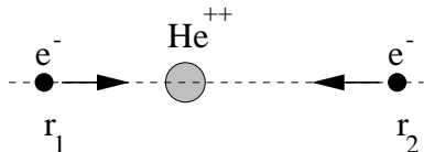
Fig. 6.2 Collinear helium, with the two electrons on opposite sides of the nucleus.
