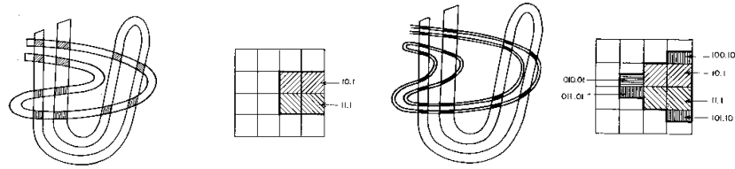
Fig. 13.2 (a) An incomplete Smale horseshoe: the inner forward fold does not intersect the two rightmost backward folds. (b) The primary pruned region in the symbol square and the corresponding forbidden binary blocks. (c) An incomplete Smale horseshoe which illustrates (d) the monotonicity of the pruning front: the thick line which delineates the left border of the primary pruned region is monotone on each half of the symbol square. The backward folding in figures (a) and (c) is only schematic - in invertible mappings there are further missing intersections, all obtained by the forward and backward iterations of the primary pruned region.
