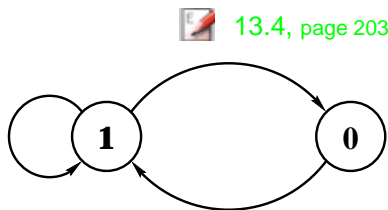
Fig. 13.1 The golden mean pruning rule Markov graph, see also Fig. 10.11.
