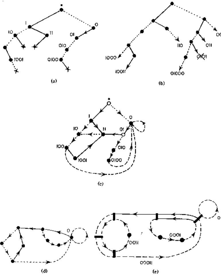
Fig. 13.3 Conversion of the pruning front of Fig. 13.3.1 (d) into a finite Markov graph. (a) Starting with the start node “.”, delineate all pruning blocks on the binary tree. A solid line stands for “1” and a dashed line for “0”. Ends of forbidden strings are marked with \times . Label all internal nodes by reading the bits connecting “.”, the base of the tree, to the node. (b) Indicate all admissible starting blocks by arrows. (c) Drop recursively the leading bits in the admissible blocks; if the truncated string corresponds to an internal node in (a), connect them. (d) Delete the transient, non-circulating nodes; all admissible sequences are generated as walks on this finite Markov graph. (e) Identify all distinct loops and construct the determinant (13.17).
