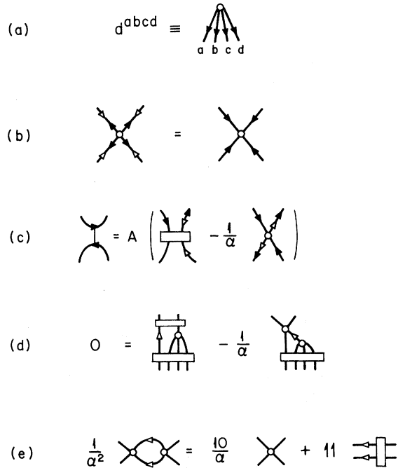
FIG. 18. (a) Diagrammatic notation for the tensor d_{abcd} for the exceptional group E_7 (56), (b) symplectic invariant tensor f^{ab} relates d^{abcd} and d_{abcd} , (c) the most general form of the gluon projection operator ( f^{ab} invariance has already been imposed), (d) Brown relation which relates contractions of pairs of d_{abcd} , (e) reduction of a one-loop diagram.
