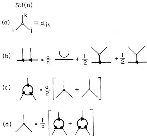
FIG. 25. (a) Notation for the (fully symmetric) numerical tensor d_{ijk} , (b) multiplication rule for SU(n) matrices T_i \equiv \frac{1}{2} g \lambda_i , (c) decomposition of three external gluon quark-loop into real and imaginary parts, (d) d_{ijk} as its real part.
