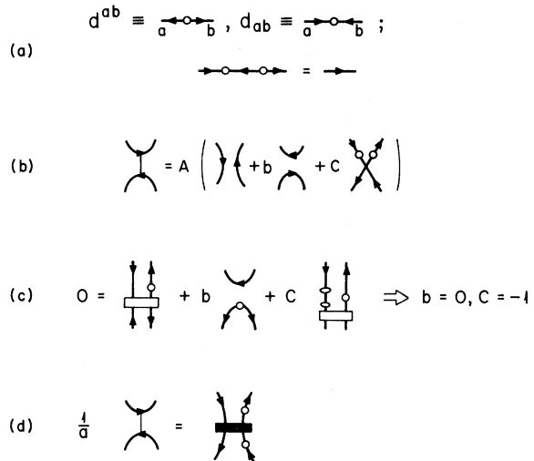
FIG. 10. (a) Diagrammatic notation for SO( n )-invariant tensor d_{ab} , (b) the most general form of the gluon projection operator for SO( n ), (c) d_{ab} invariance condition, (d) gluon projection operator for SO( n ).
